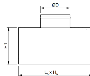
Vertical connection (opposite exit)
