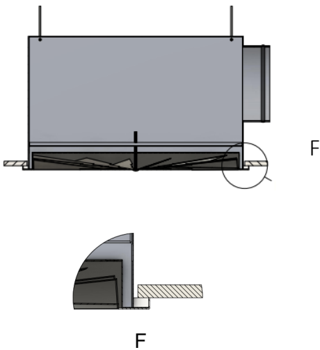
Installation in continuous ceiling
