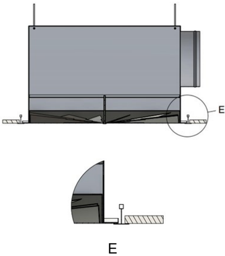
Installation in T-bar suspended ceiling
