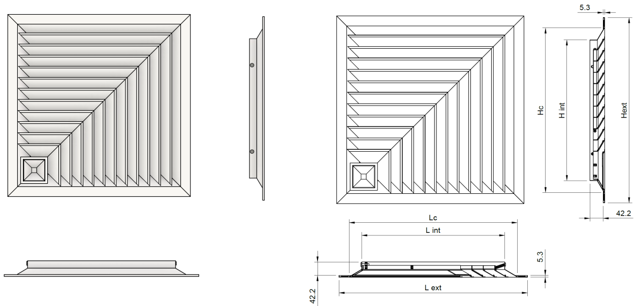
Ceiling diffuser dimensions
