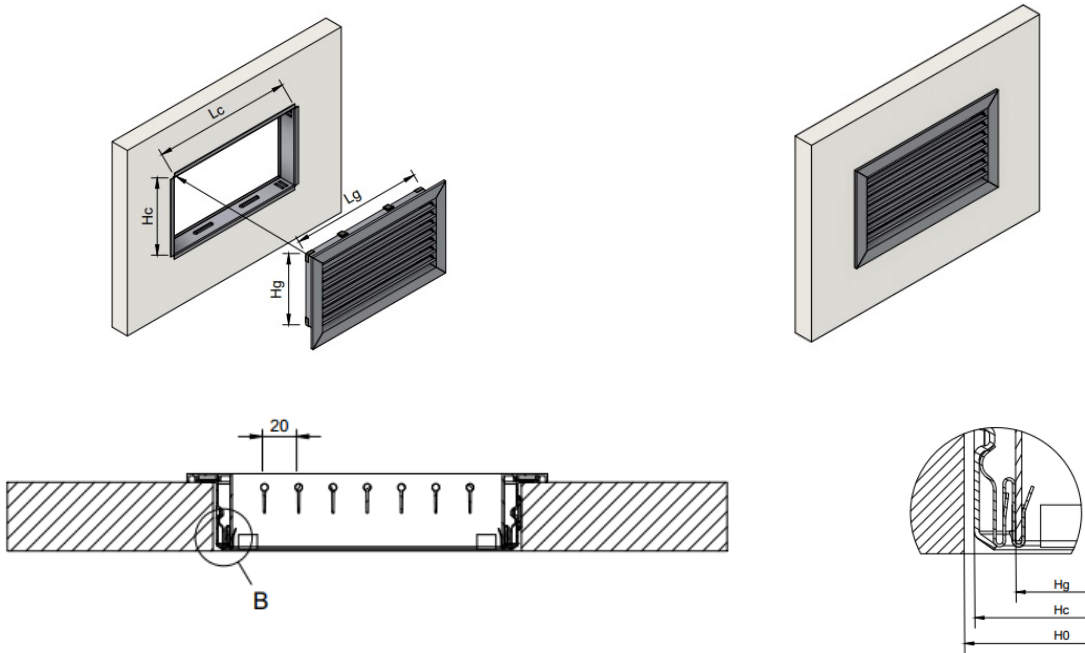
Installation in T-bar suspended ceiling DD-I 595X595 mm (external size)
