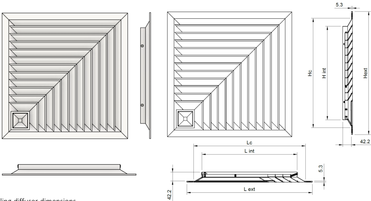
Ceiling diffuser dimensions
